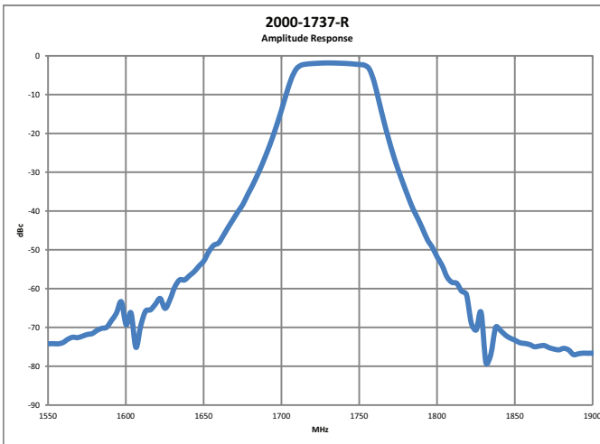
Passband
