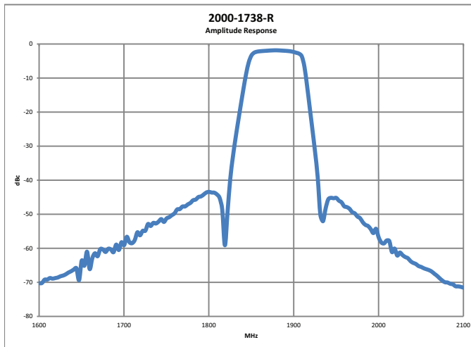
Passband
