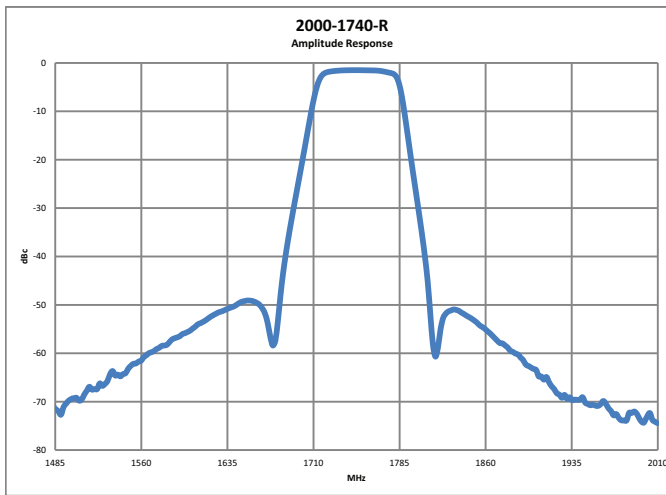
Passband
