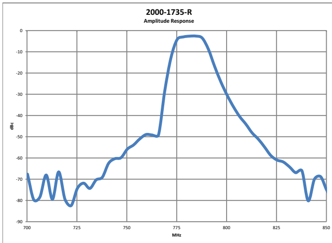
Passband
